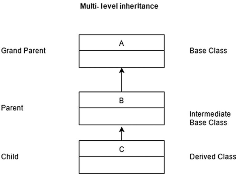
Figure 3-2. Multi-level inheritance
