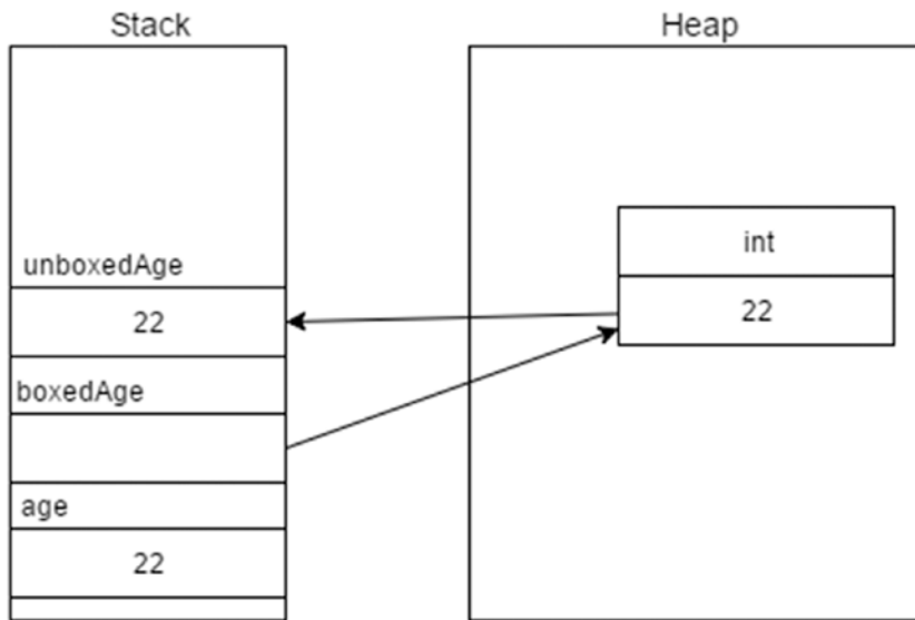
Figure 4-2. Unboxing
