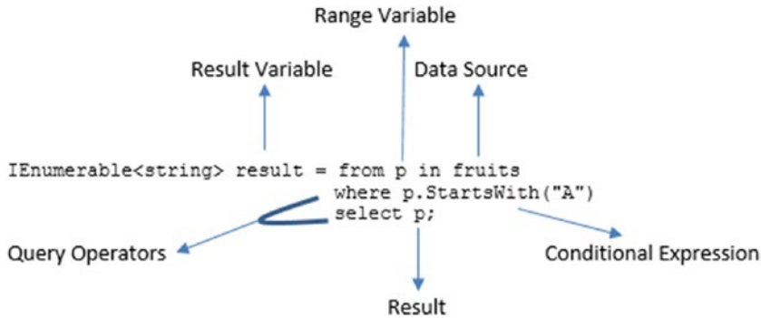
Figure 6-2. Query Syntax
