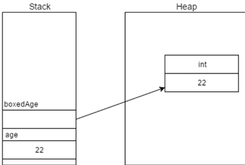
Figure 4-1. Boxing
