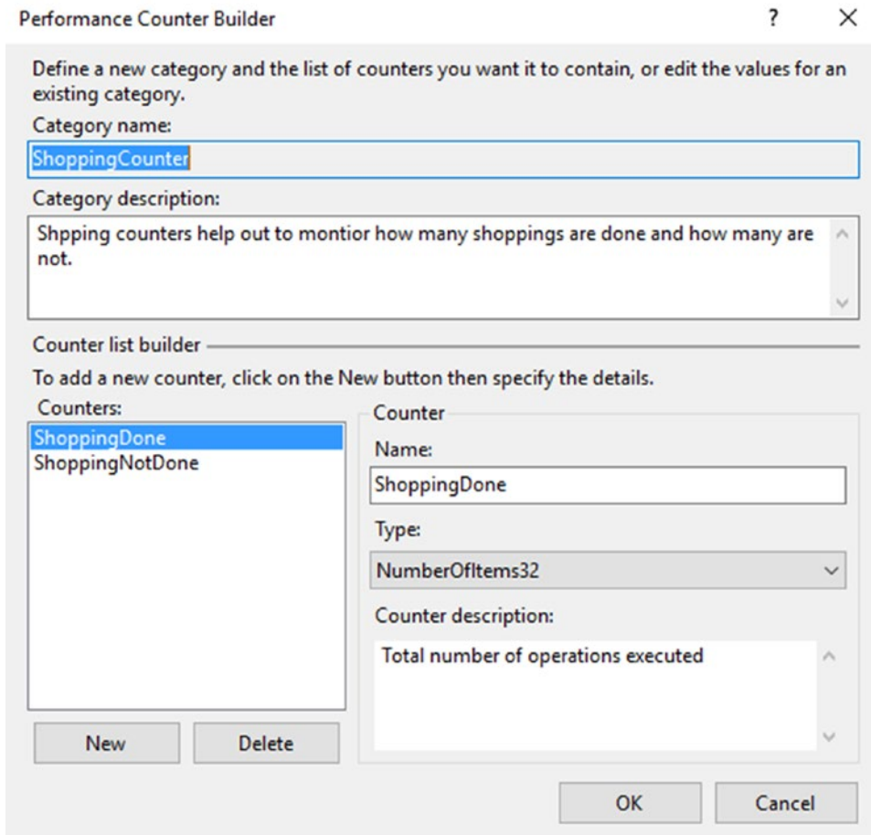
Figure 15-12. Performance Builder
