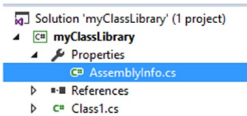
Figure 14-6. AssemblyInfo.cs
