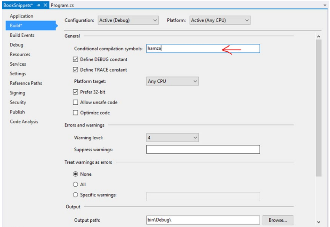
Figure 15-4. Project properties
