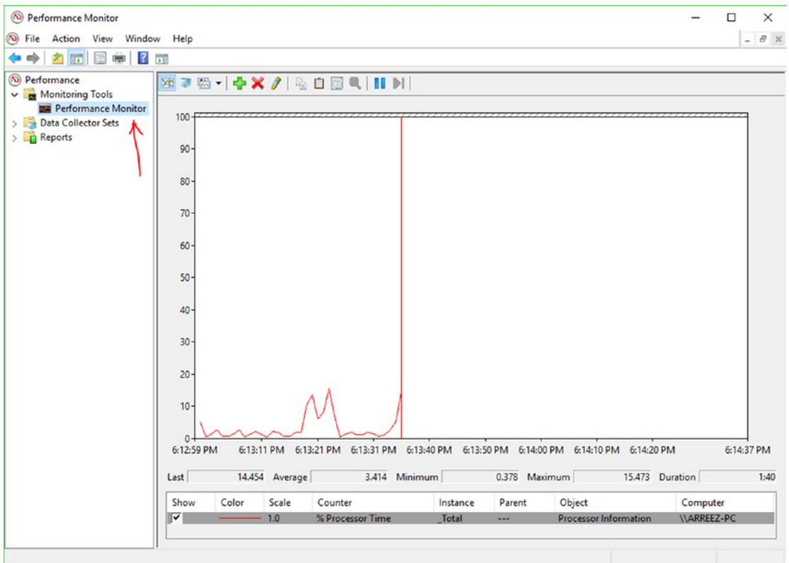
Figure 15-10. Performance Monitor
