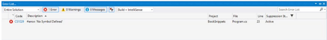
Figure 15-5. Error list
