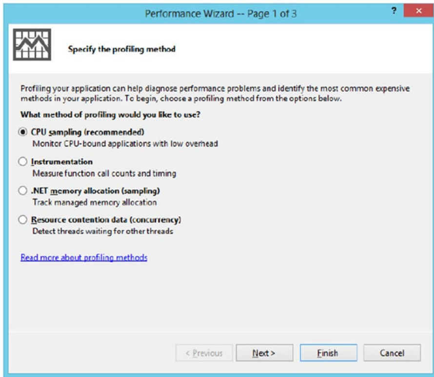
Figure 15-8. Performance Wizard
