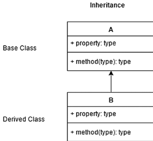
Figure 3-1. Inheritance
