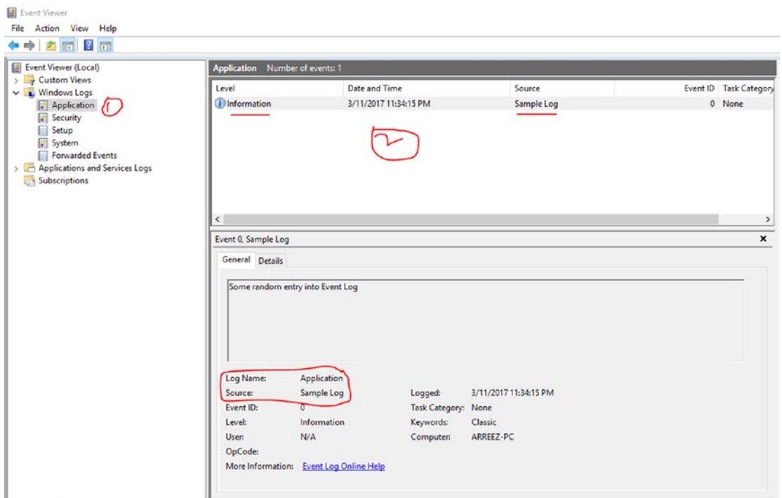
Figure 15-7. Event viewer
