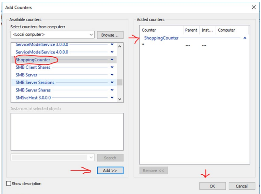
Figure 15-13. Add Counters
